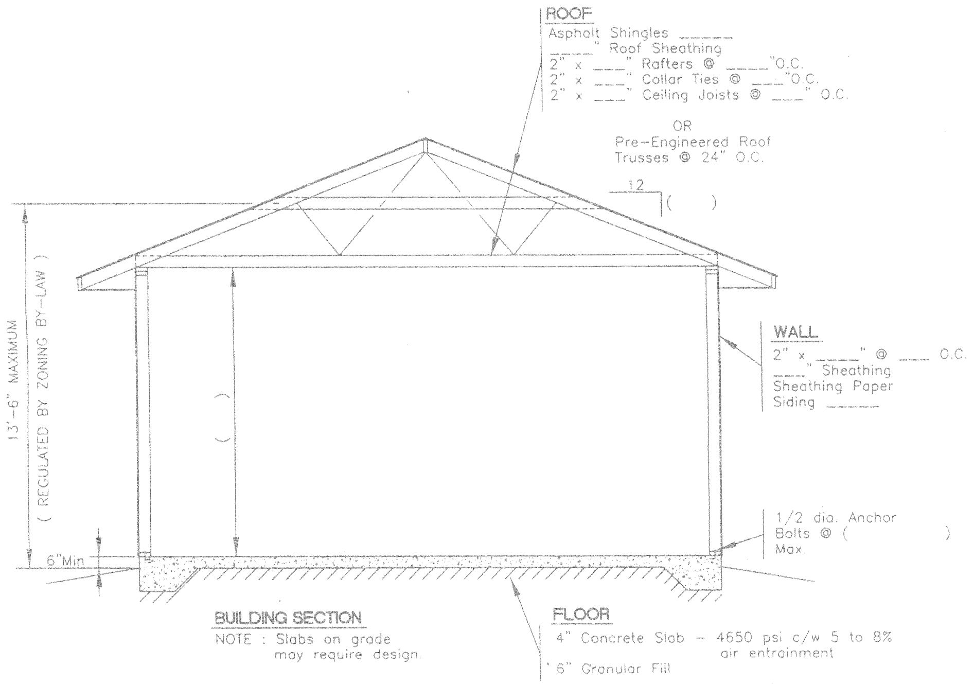
SAMPLE PRIVATE ONE STOREY GARAGE PLAN This sample is intended to assist the Applicant in preparing their plan of Proposed Construction
